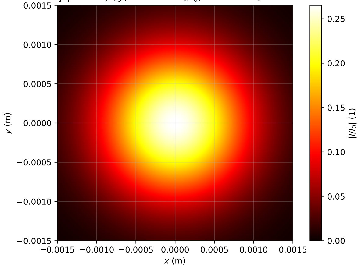
Intensity profile I(x, y, z = 3.821m)/I_0 , P_{in}=0.2P_{cr} , artificial time
